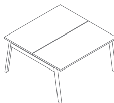
BOB44 1400 / 1410 / 740 61.2 kg
